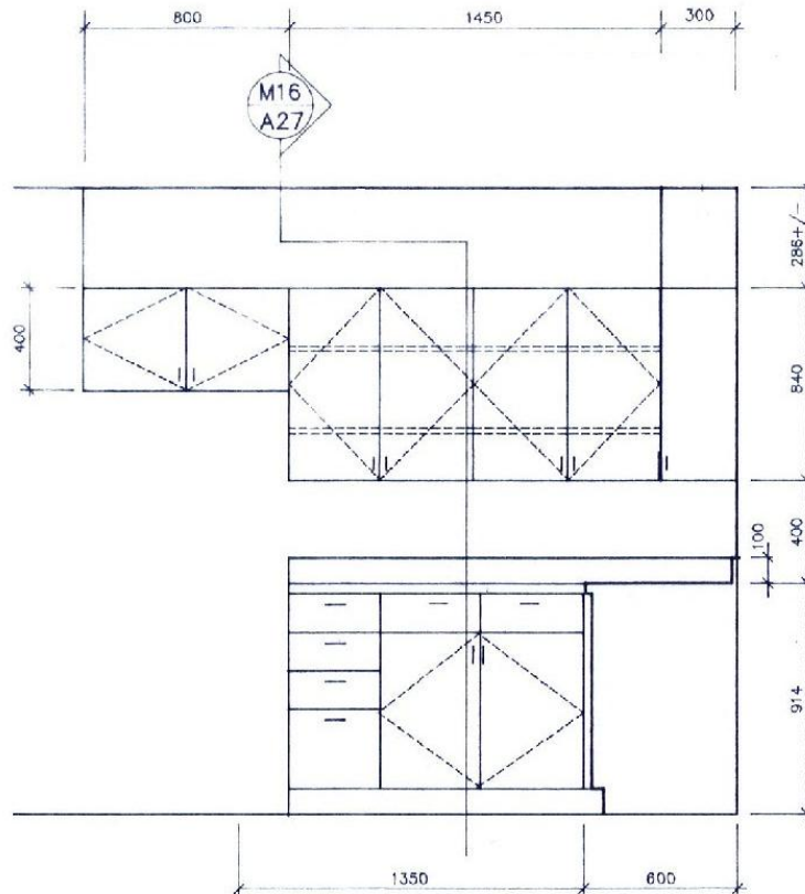
All Units - Existing Cabinet Layout
