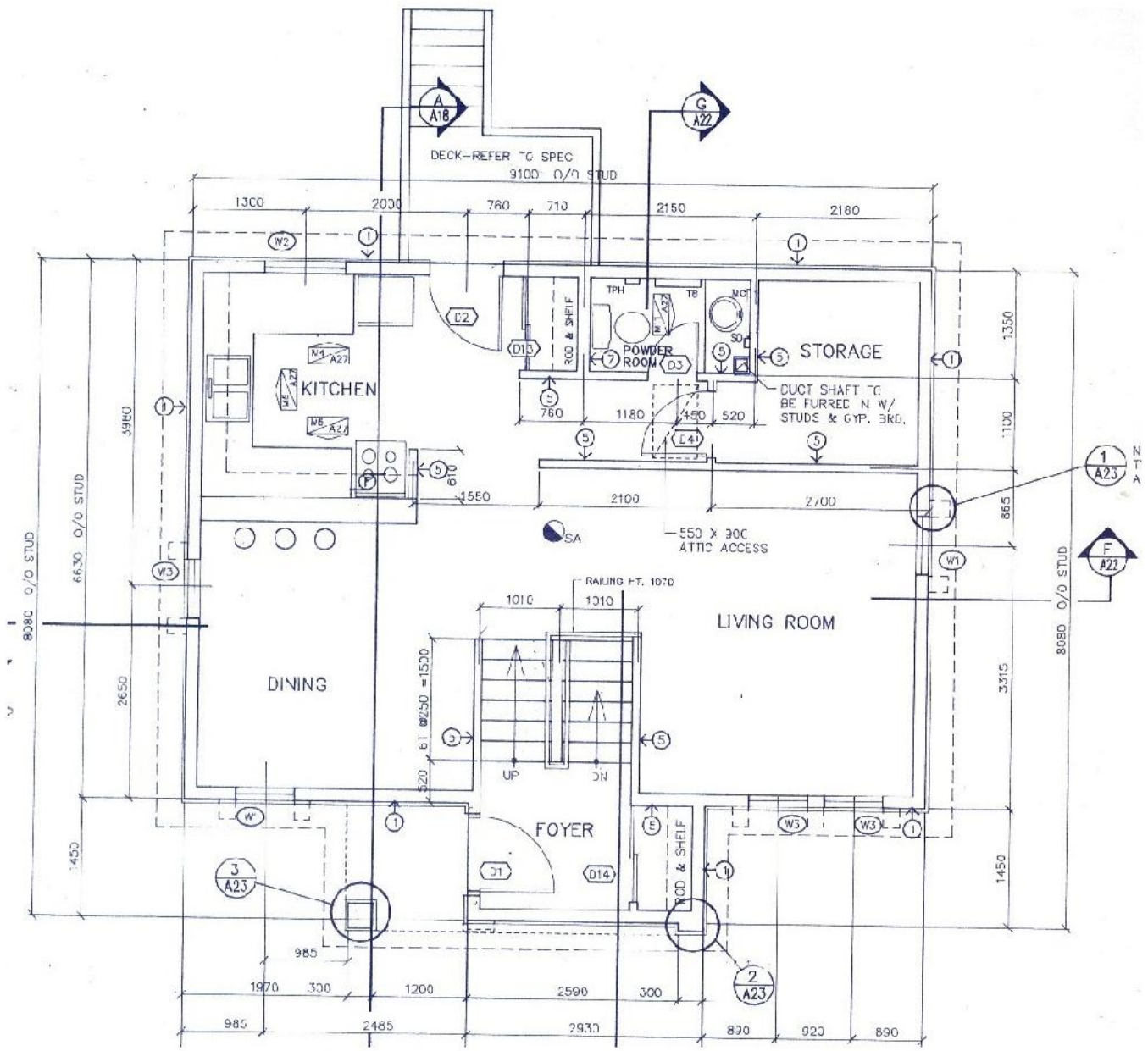
All Units - Upper Floor Plan
